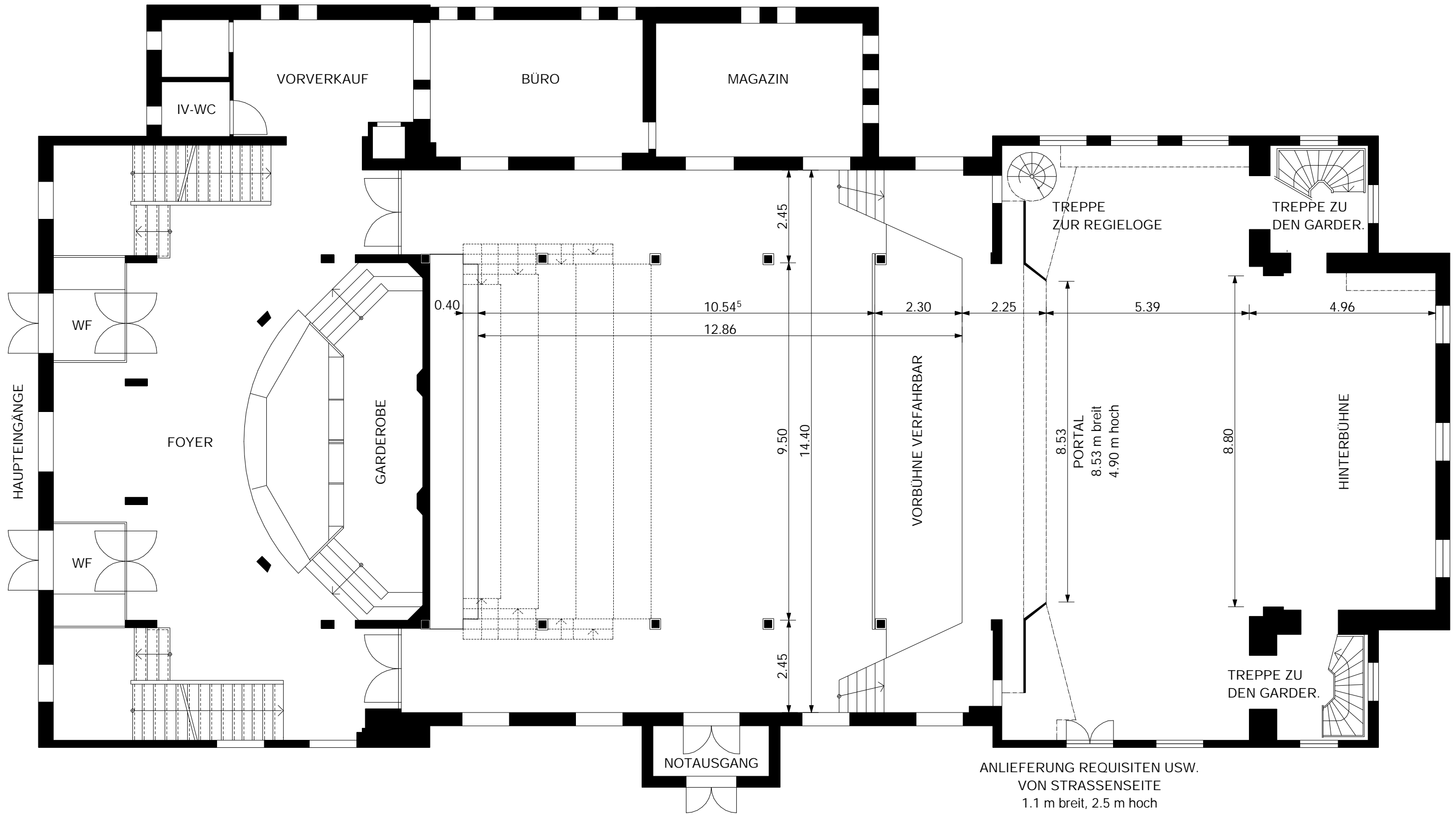
Tonhalle Wil "Theatersaal" 1:100
